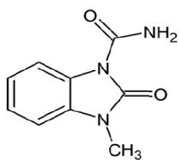
3-Methyl-2-Oxo-Benzimidazol-1-Carboxamid
