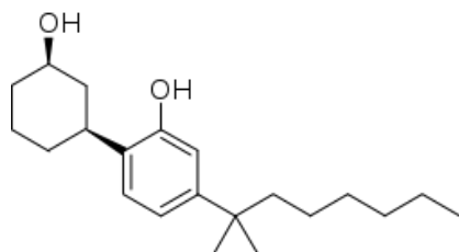
3-[4-(1,1-Dimethylheptyl)-2-hydroxy-Phenyl]- Cyclohexanol
