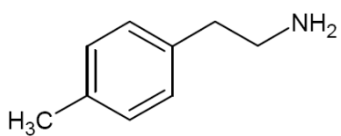
2-(4-Methylphenyl)-Ethanamin
