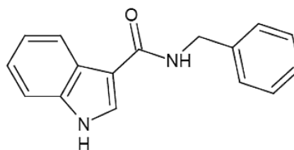
N-Benzyl-Indol-3-Carboxamid
