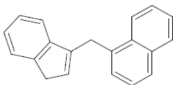
1-(1H-Inden-3-yl-Methyl)-Naphthalen
