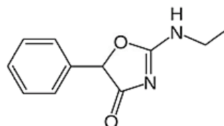
2-Ethylamino-5-Phenyl-1,3-Oxazol-4-on
