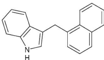
3-(Naphthalen-1-yl-Methyl)-1H-Indol
