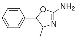
4-Methyl-5-Phenyl-2-Amino-Oxazolin
