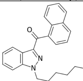
1-Naphthalen-yl-(1-Pentyl-Indazol-3-yl)- Methanon
