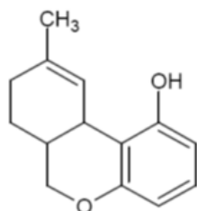
9-Methyl-tetrahydro-6H-Benzo[c]Chromen-1-ol
