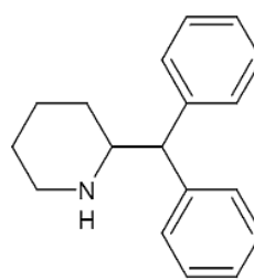
2-(Diphenylmethyl)-Piperidin
